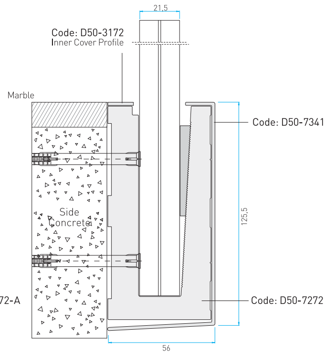
Direct mounting to the side Wall
