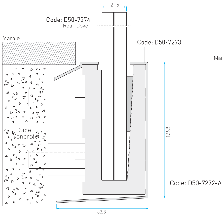
Distant mounting according to marble distance
