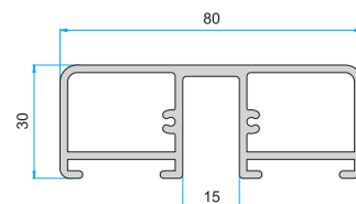
Code: PR-7116 On-Glass Profile
