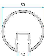
Code: PR-5148 Glass Fixing Accessory
