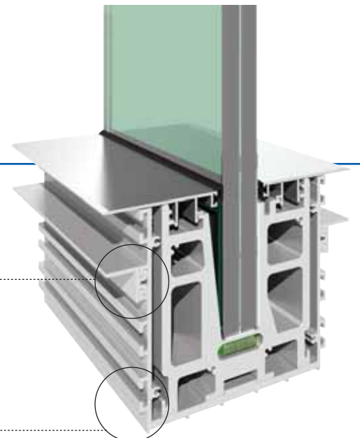
Height Adjusting U Case Profile Option
