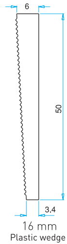
16 mm Plastic wedge
